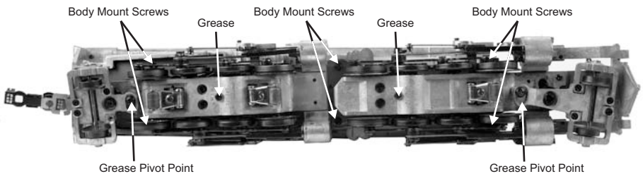
Figure: Body Mount Screws and Grease Points
