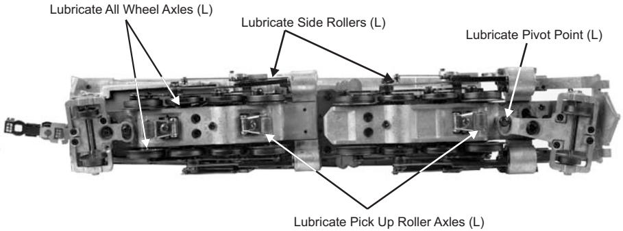
Figure: Lubricating the Locomotive
